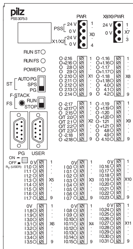
Fig. 7-1: Terminal configuration on programmable systems from the PSS 3075-3 series (Example: PSS 3075-3)
